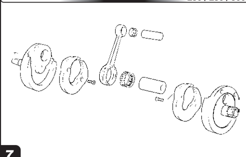
Cigüeñal / Crankshaft GAS GAS TXT PRO 06 250 / 280 / 300
